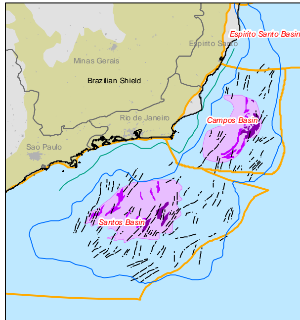
Brazil Pre-Salt Basins
