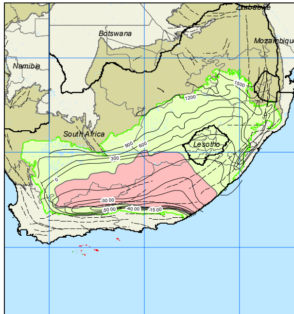
Karoo Basin Shale Gas Potential
