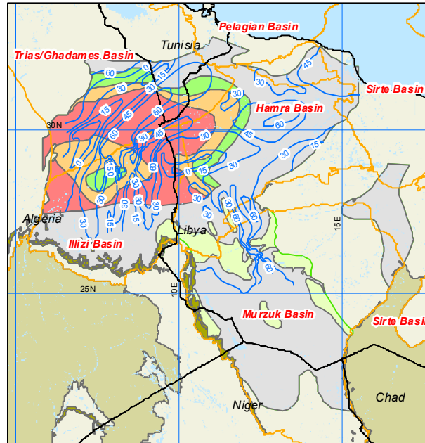
Tannezuft Hot Shale Isopach & Maturity
